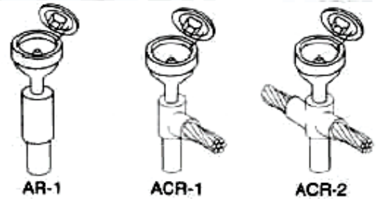
CABLE & AIRCRAFT GROUNDING RECEPTACLE TO GROUND ROD
