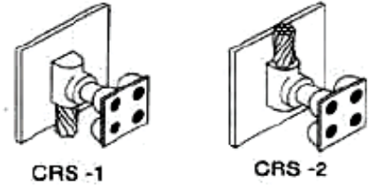
CABLE & GROUND PLATES TO STEEL
